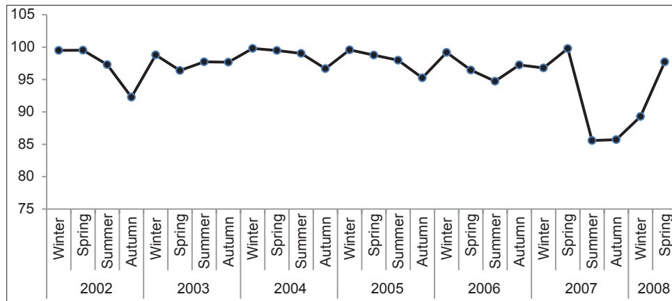
Figure 2: Turbidity removal efficiency in Parsabad WTP in the study period
